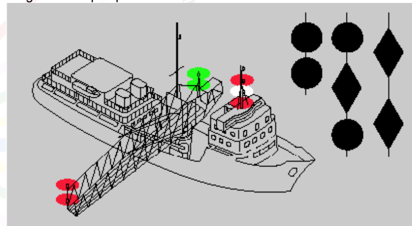
Vessel engaged in dredging or underwater operations when restricted in ability to maneuver- not making way with an obstruction on the starboard side. Same for International.
