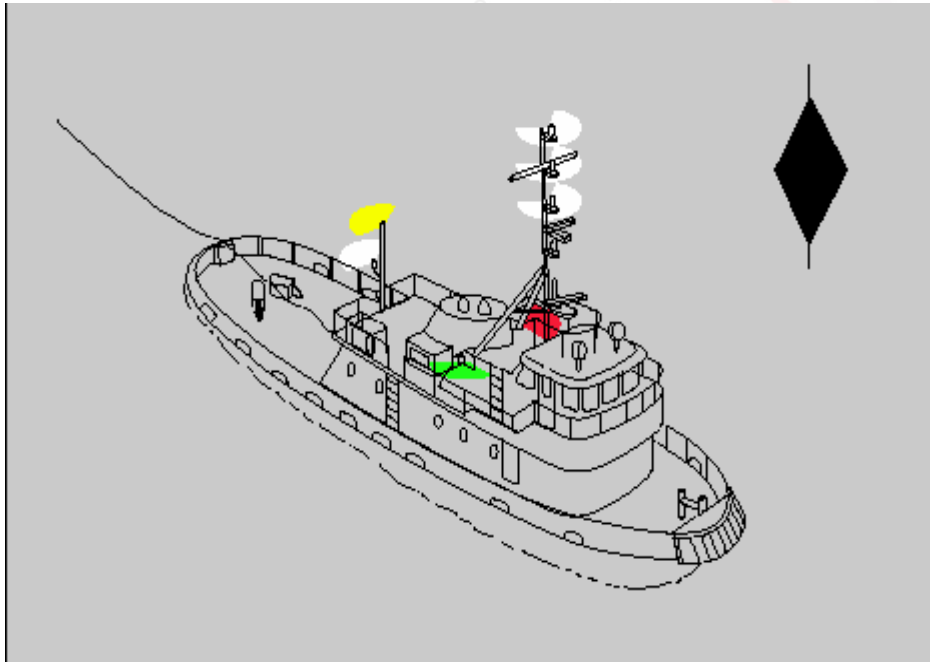
Power-driven vessel towing astern - towing vessel less than 50 meters in length; length of tow exceeds 200 meters. Same for Inland
