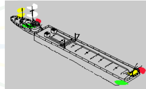
Vessel being pushed ahead, not being part of a composite unit.
