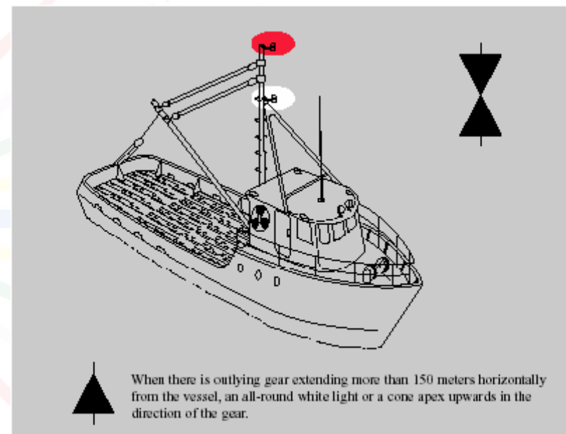
Vessel engaged in fishing other than trawling--not making way. Same for International.
