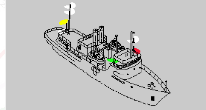
Power-driven vessel towing astern--length of tow 200 meters or less. When masthead lights for towing or pushing are exhibited aft, a forward masthead light is required. Same for International.
